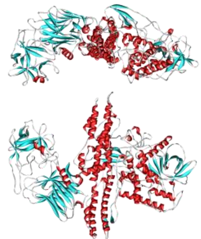
Structure of a botulinum toxin molecule. 1
